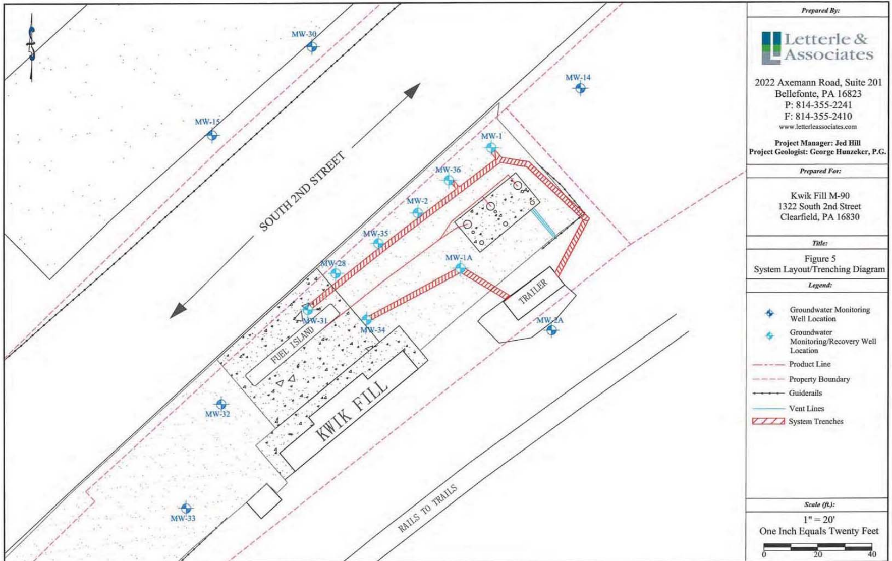
Figure 3 – Remedial System Layout
