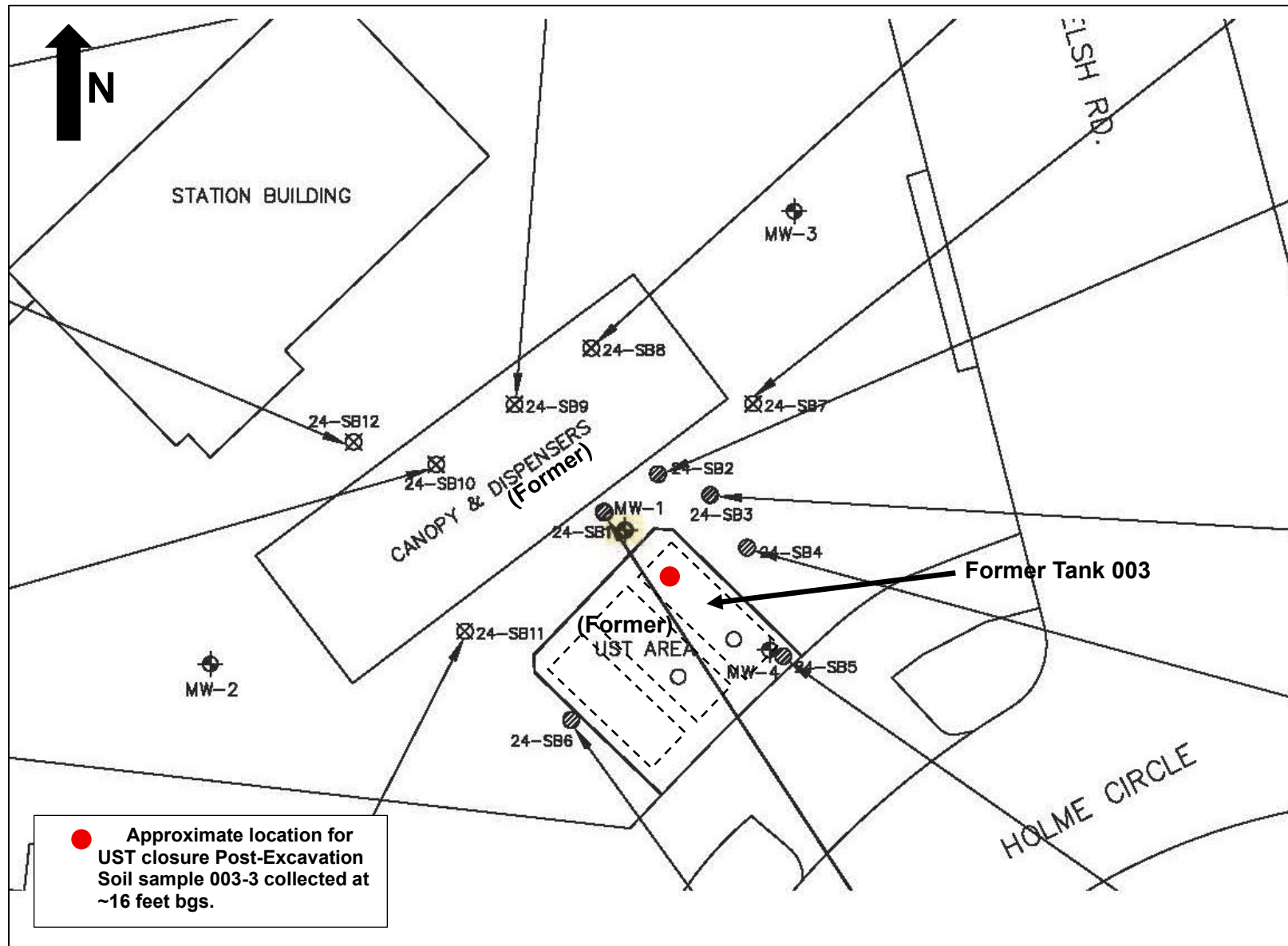
Figure 2 – Soil Boring Locations
