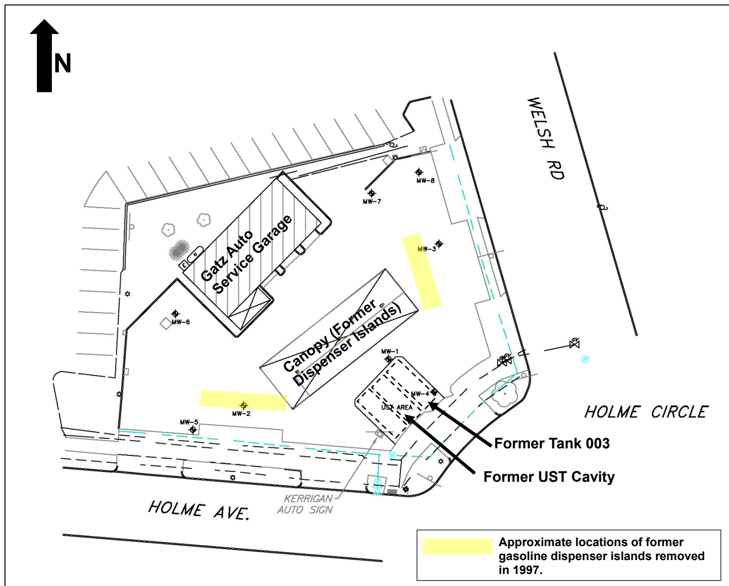
Figure 2 – Former UST System & Existing Monitoring Well Locations
