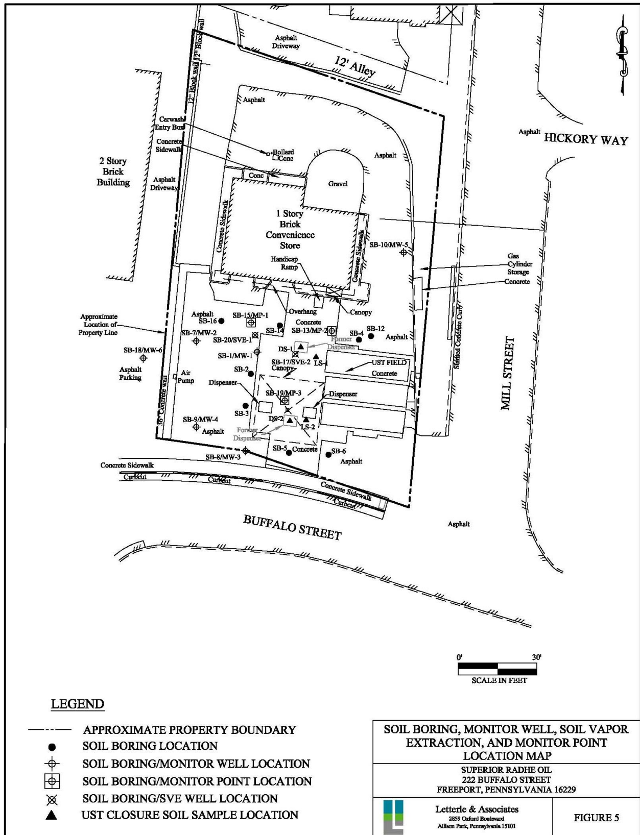
FIGURE 3 – SOIL BORING & MONITORING WELL LOCATIONS
