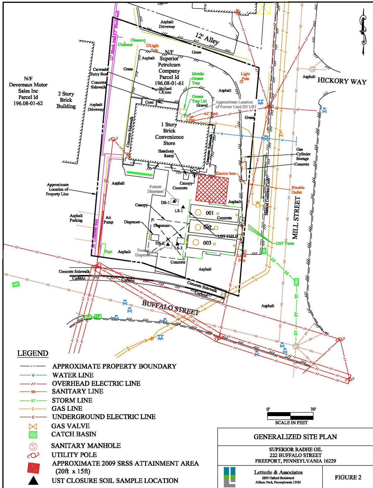
FIGURE 2 – SITE LAYOUT
