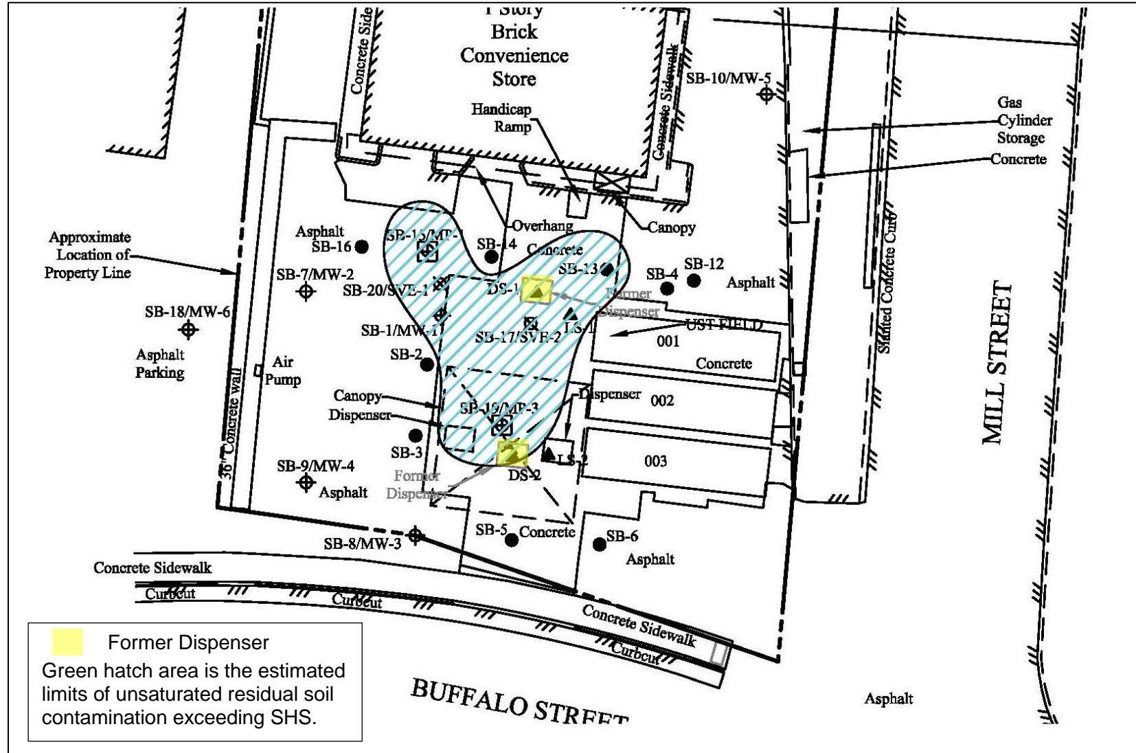
FIGURE 4 – ESTIMATED EXTENT OF UNSATURATED SOIL IMPACTS
